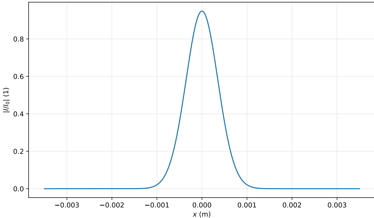
Intensity profile I(x, y = 0, z = 0.557m)/I_0 , P_{in}=0.1P_{cr} , artificial time
